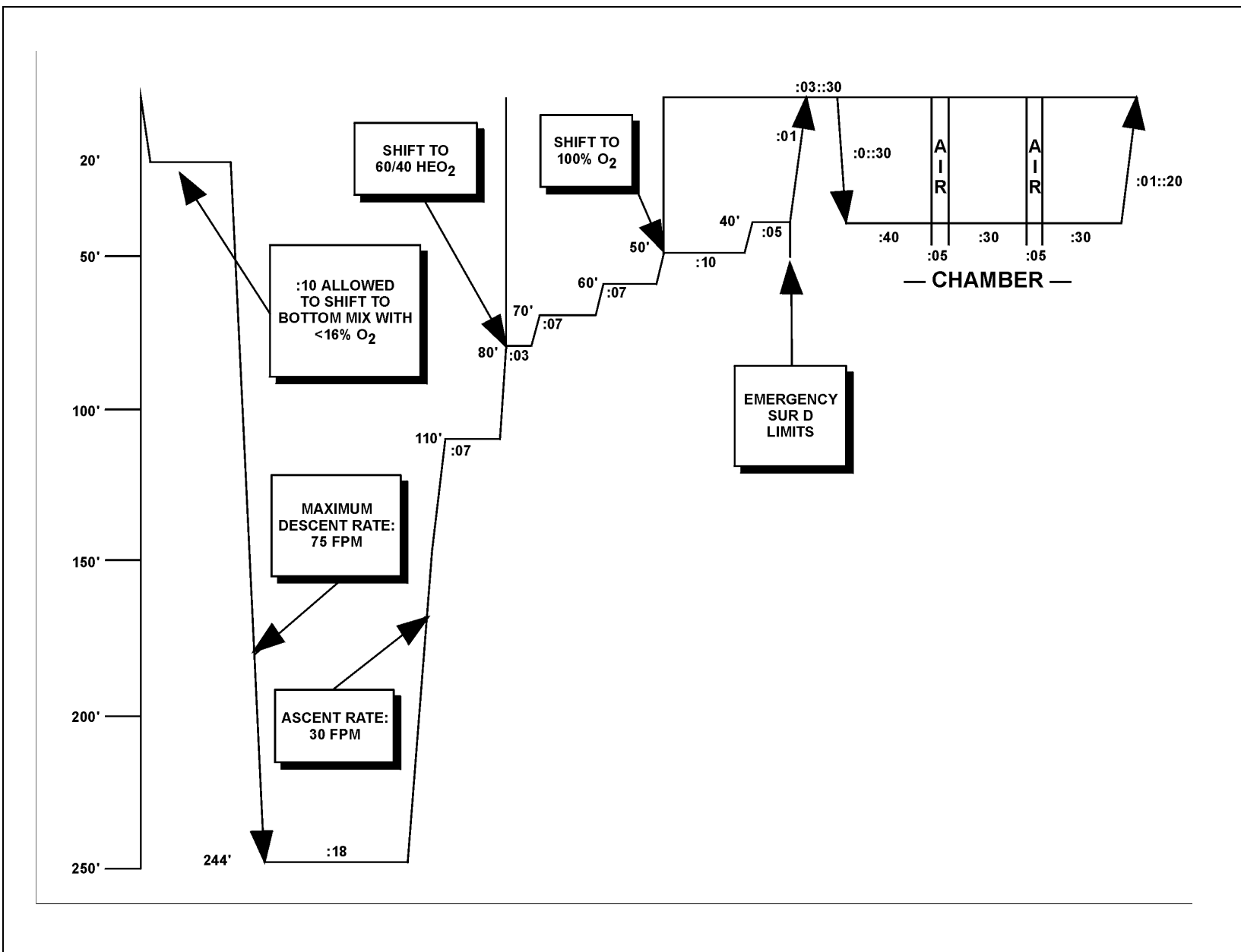
Figure 14-6. Emergency Surface Decompression Dive Profile for a 249 fsw/:18 Dive.
